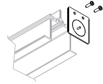
Recessed End Cap - Track jacket sold separately (ASL-FTP-241*)
