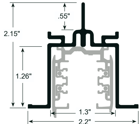
ASL-2 Series Recessed Track Jacket
