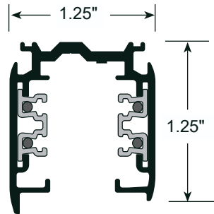
ASL-2 Series Track
