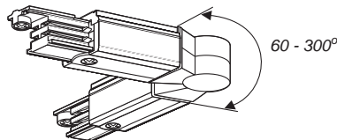
Adjustable Connector (ASL-224*)
