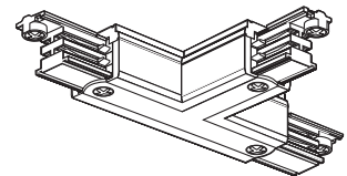
Feed-Able T Connector - Adjustable Left Polarity (ASL-240*)
